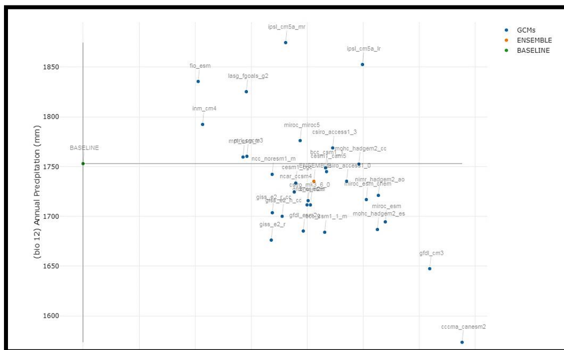
Figure 41. Example output scatterplot for variation from present. Baseline climate for temperature (x-axis) and precipitation (y-axis) indicated by green marker at left. Mean values for all projected GCMs in the region of interest are blue markers on the scatterplot (mean of all projections indicated by orange maker).
