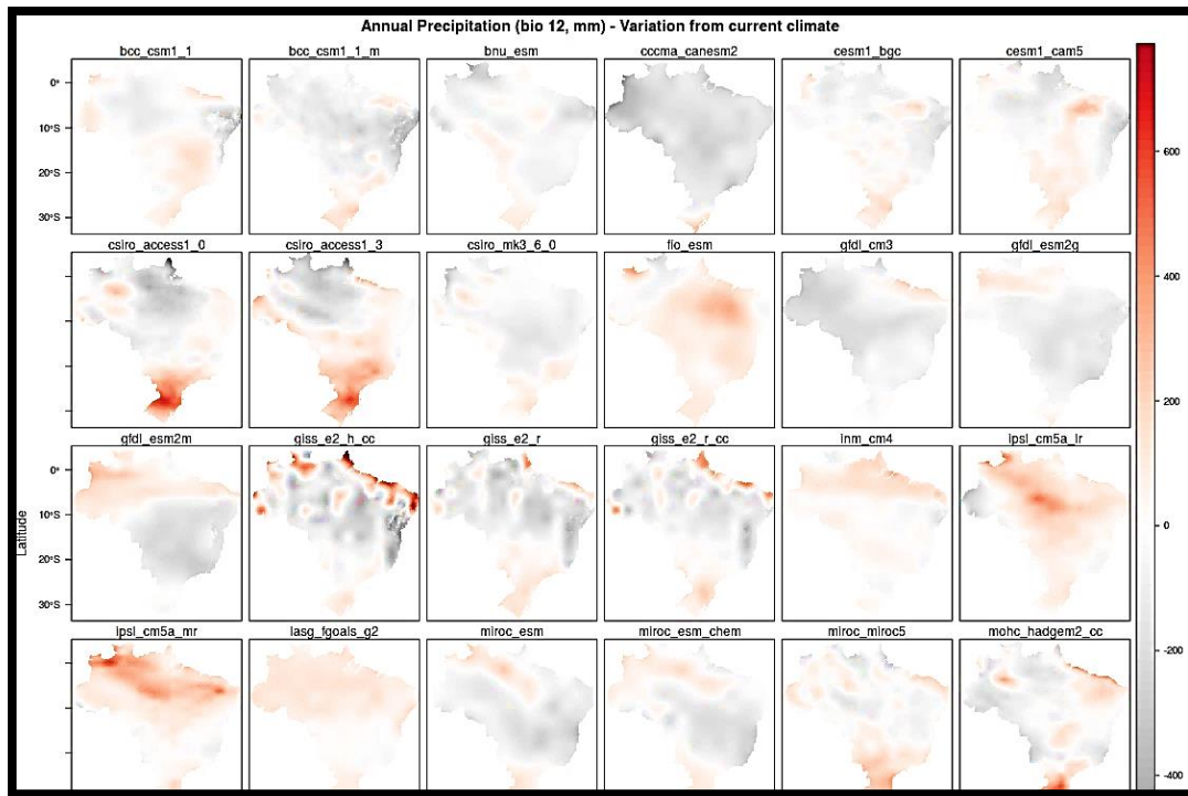
Figure 42. – Example mapped output from GCMCompareR showing the spatial variation of projected changes in annual precipitation for Brazil.
