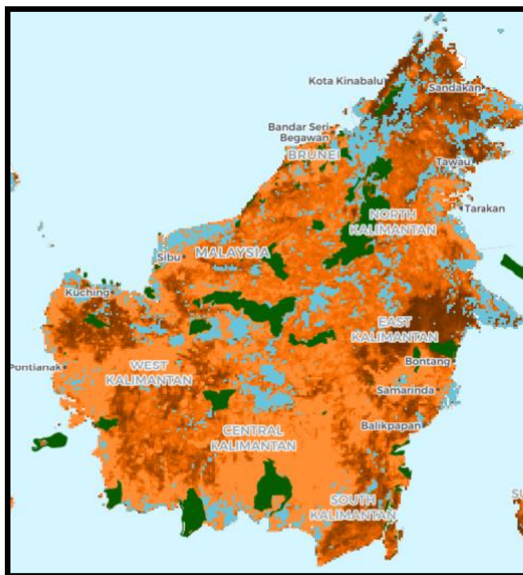
Figure 36. Screenshot of SPARC visualizer with Asia conservation priorities (blue) under climate change and total carbon stock (orange to brown color ramp) layers enabled. Zoom in on Island of Borneo.
